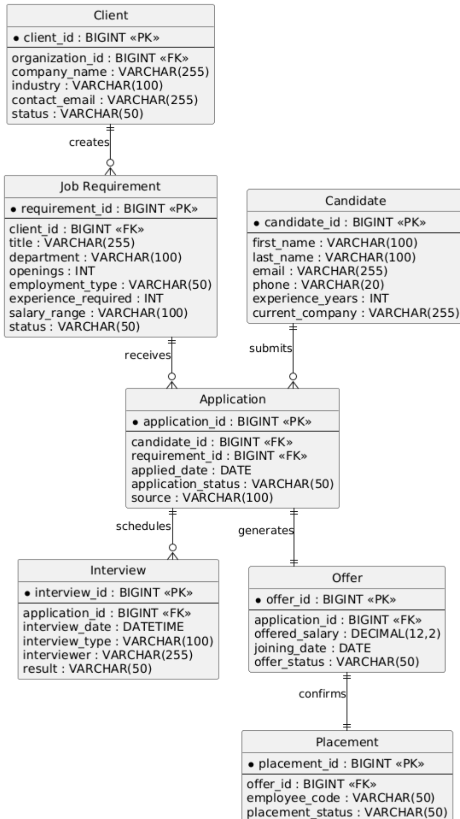
Recruitment Service Entity Relationship Diagram
