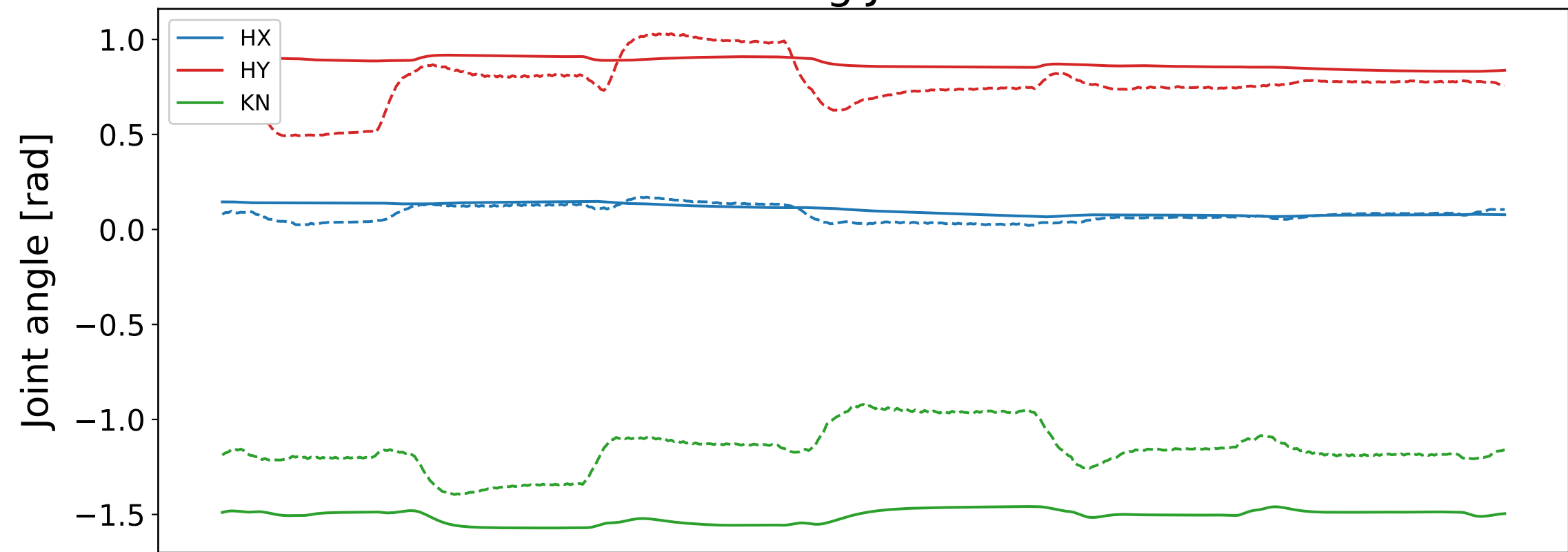
Front Left Leg Joint Positions
