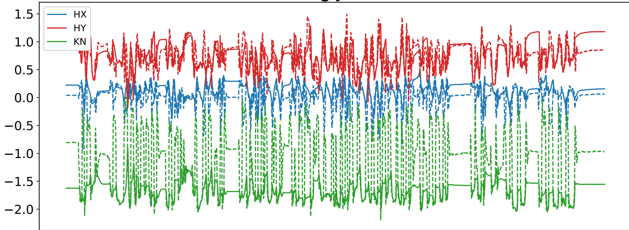
Front Left Leg Joint Positions
