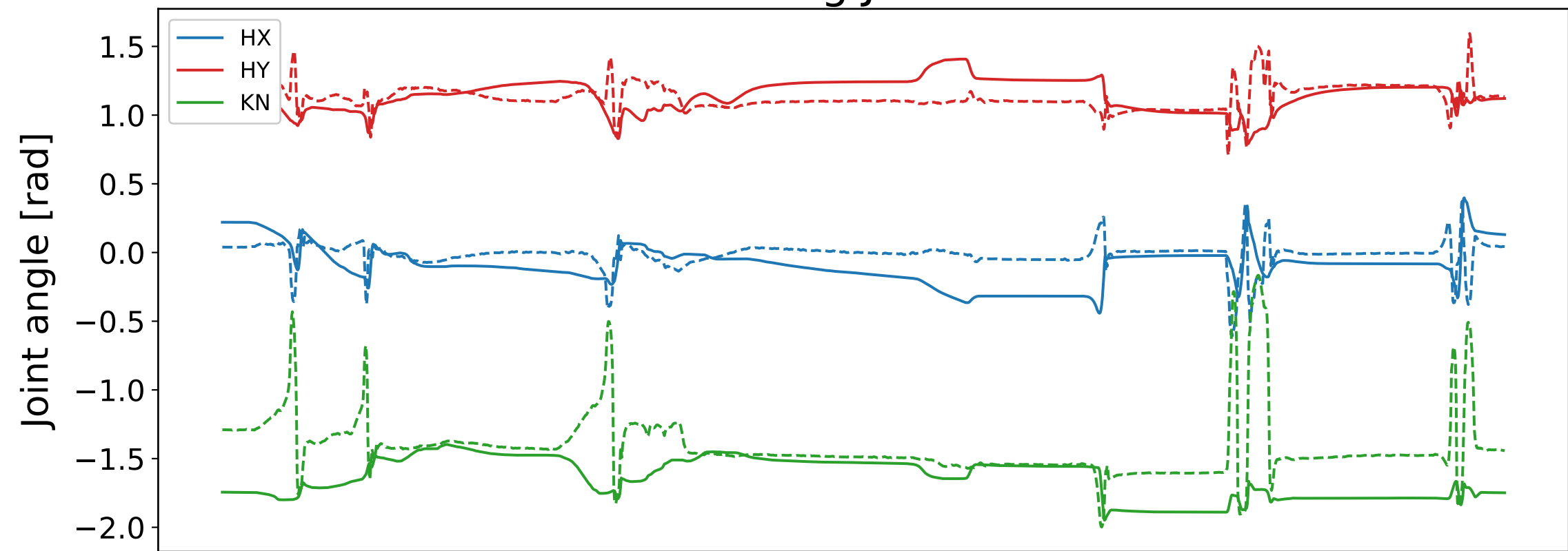
Hind Left Leg Joint Positions
