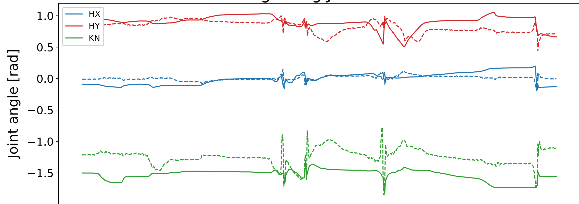
Front Right Leg Joint Positions
