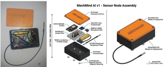
Figure 1: Assembled MechMind AI Node (NODE-001) with magnetic base, Li-ion circuit, and thermal probe.
