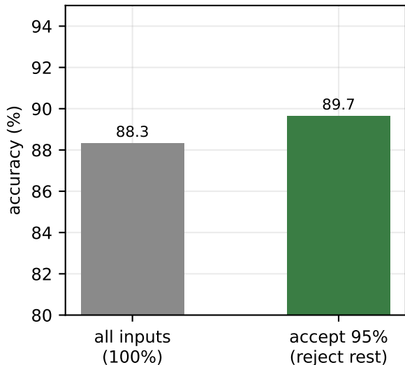
Selective prediction (PapayaFormer, u \leq \tau )
