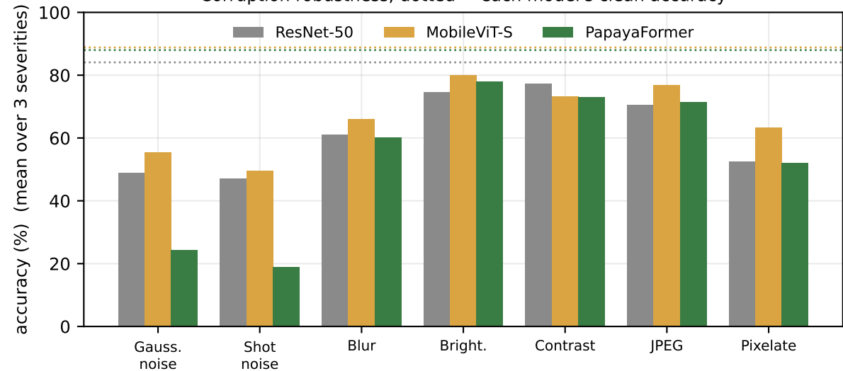
Corruption robustness; dotted = each model's clean accuracy
