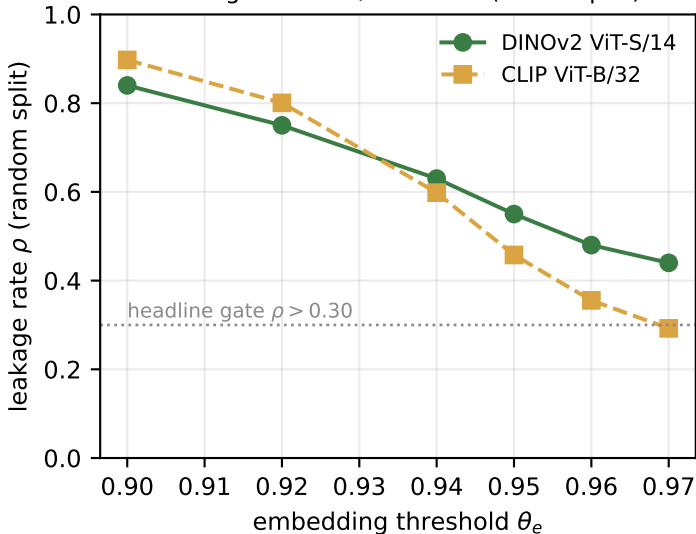
Leakage rate vs. \ threshold (raw corpus)
