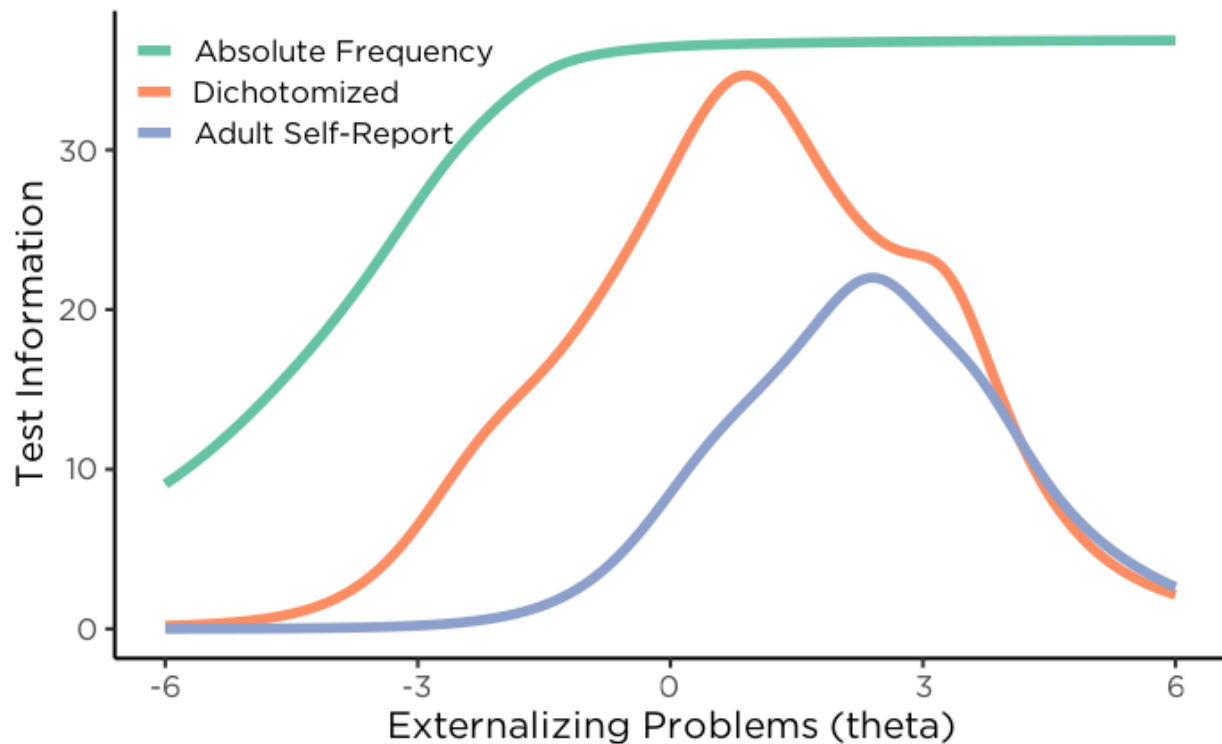
Figure 7: Test Information Functions of Absolute Frequency Versus Dichotomized Versus Adult Self-Report Items: Test Information as a Function of Theta ( \theta )
