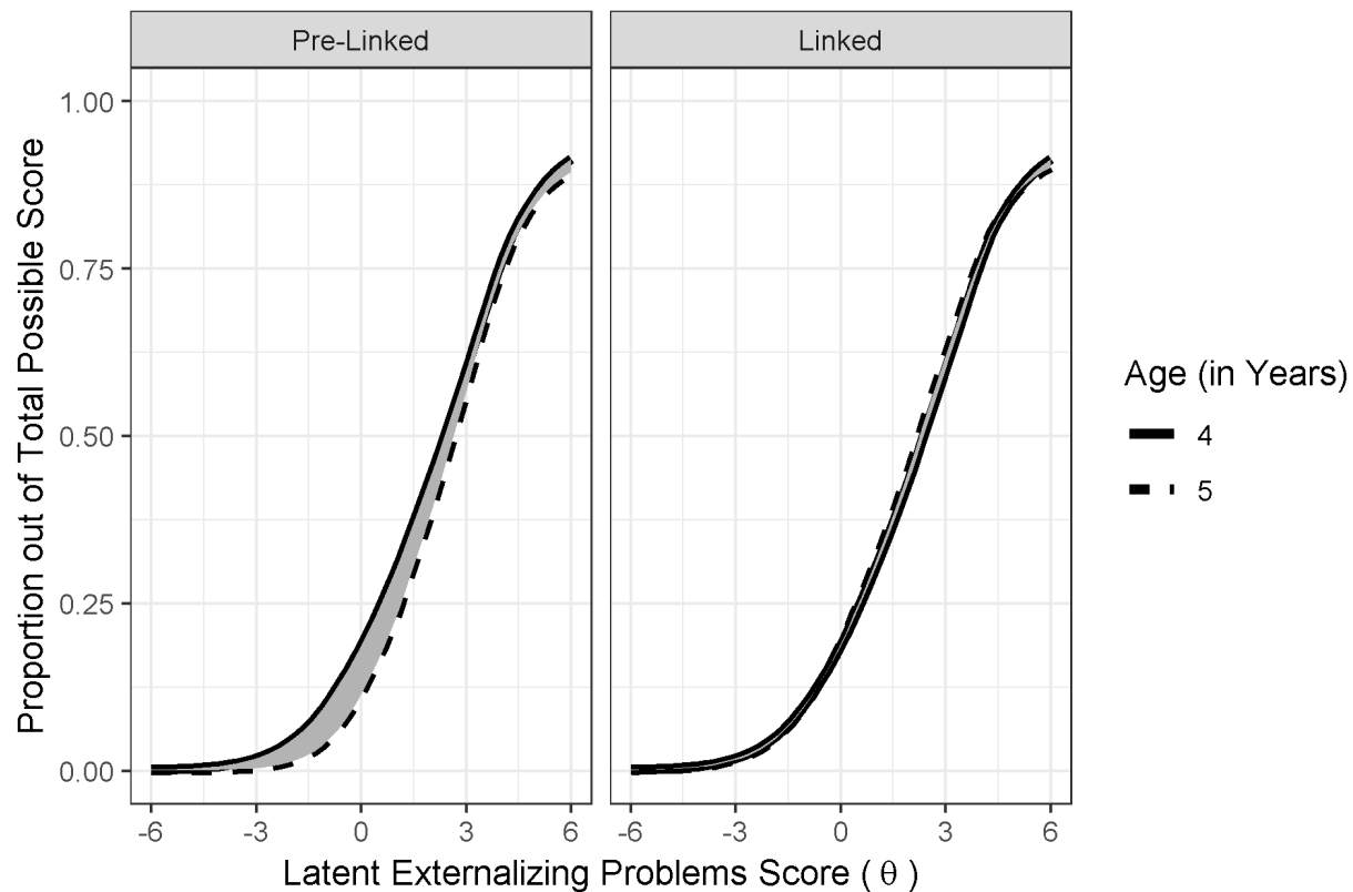
Figure 9: Example of Linking Scores From Measures Across Ages Using the Item Response Theory Approach to Developmental Scaling
