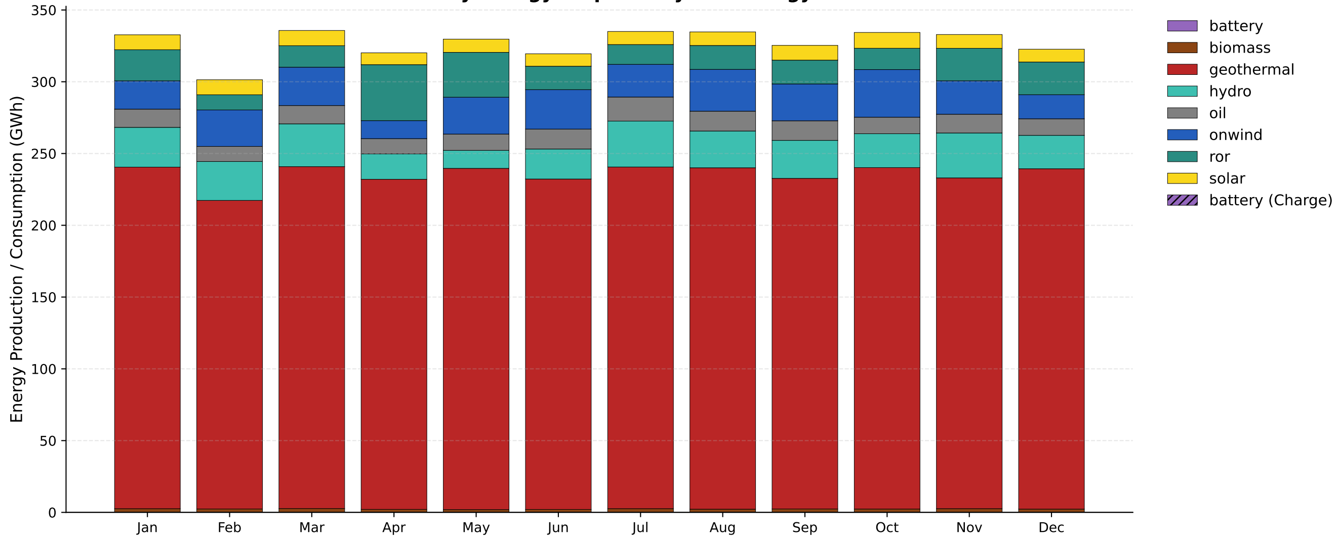
Monthly Energy Dispatch by Technology
