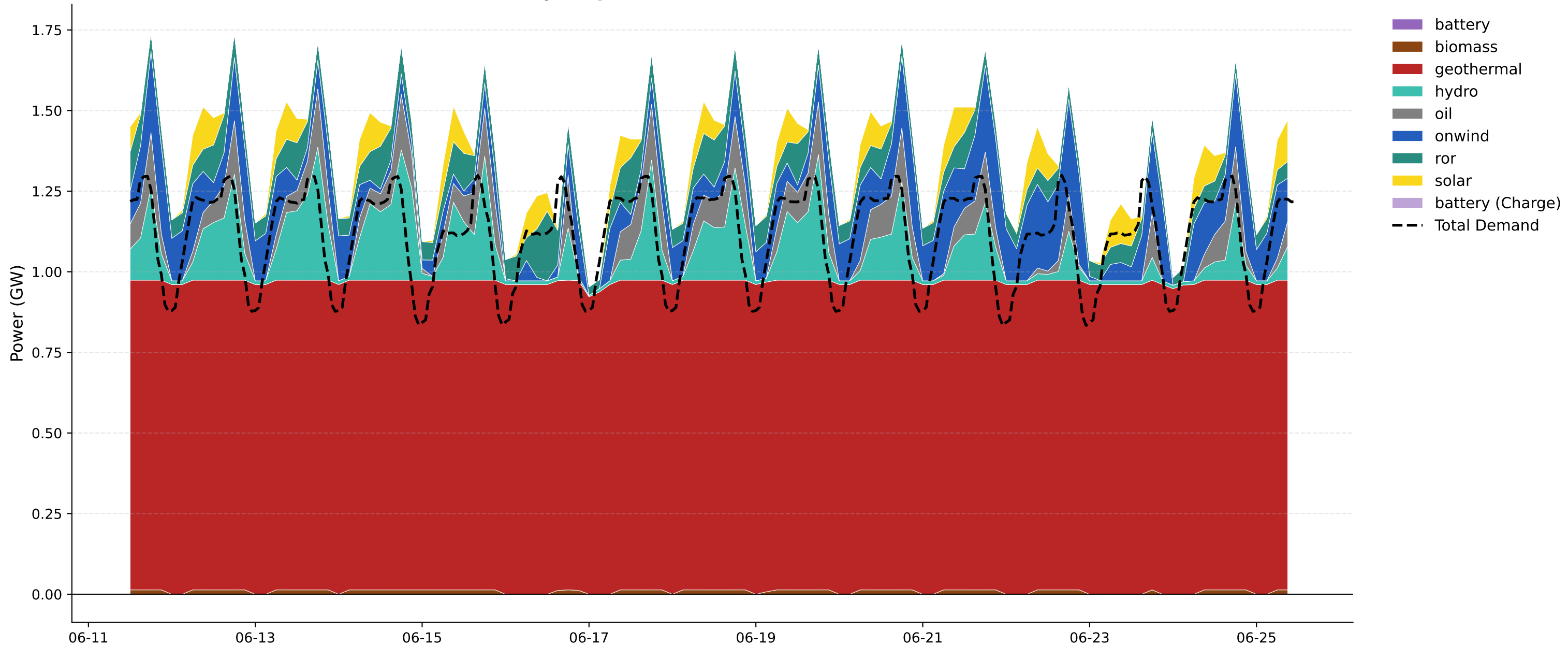
14-Day Dispatch Profile (June 11 - June 25)
