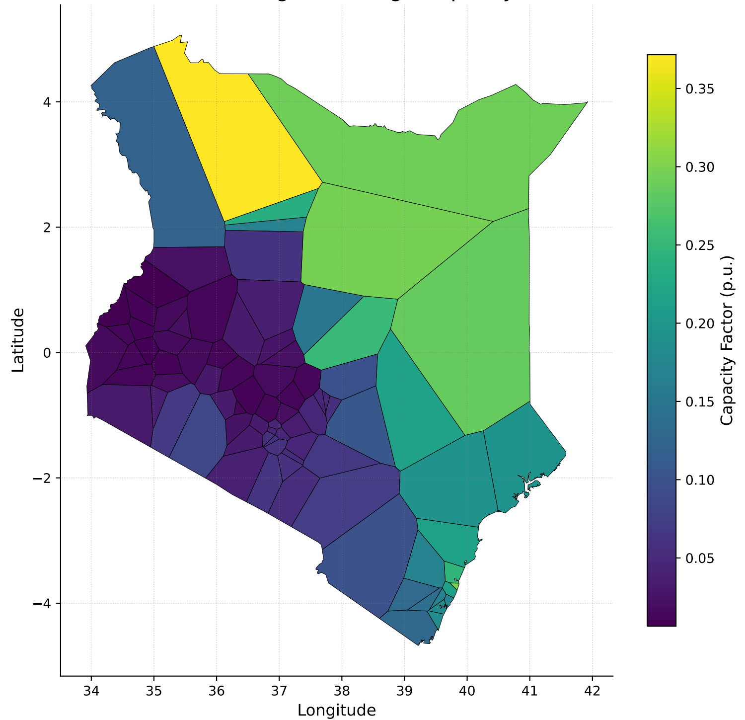
Onshore Wind: Region-Average Capacity Factor
