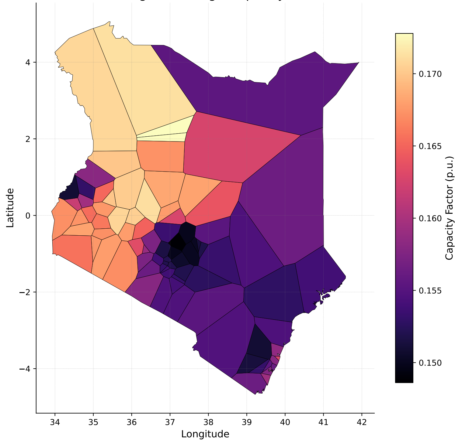
Solar: Region-Average Capacity Factor
