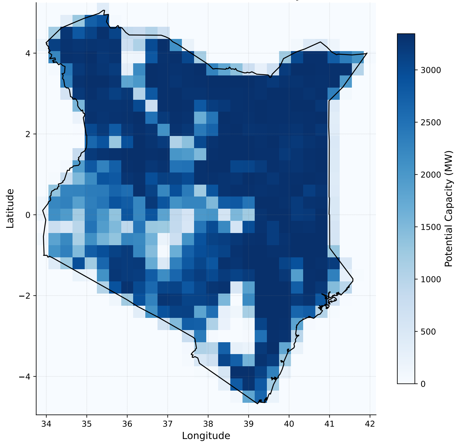
Onshore Wind: Max Potential Layout
