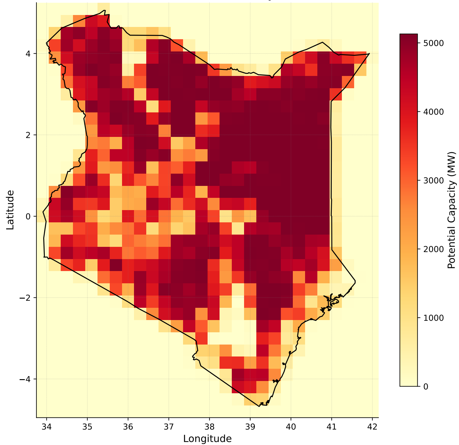
Solar: Max Potential Layout
