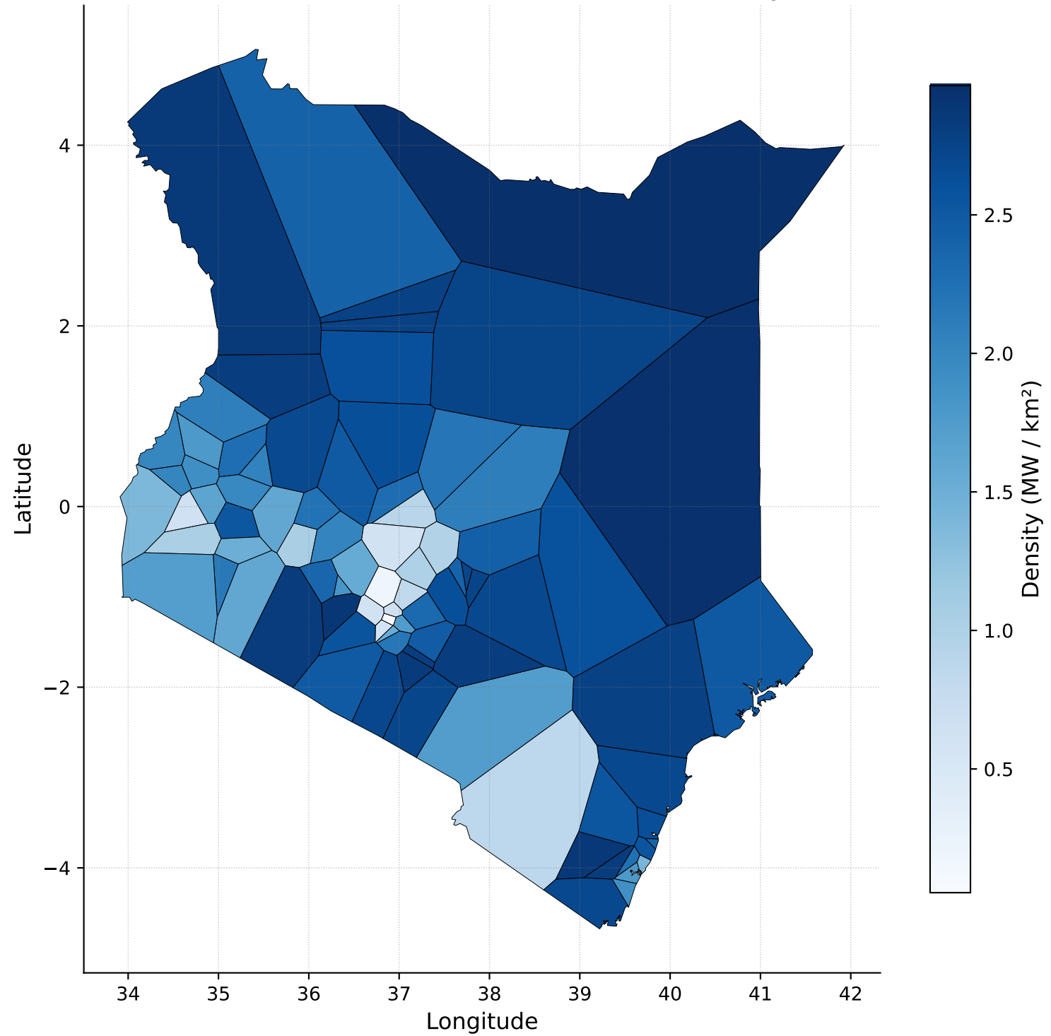
Onshore Wind: Voronoi Potential Density
