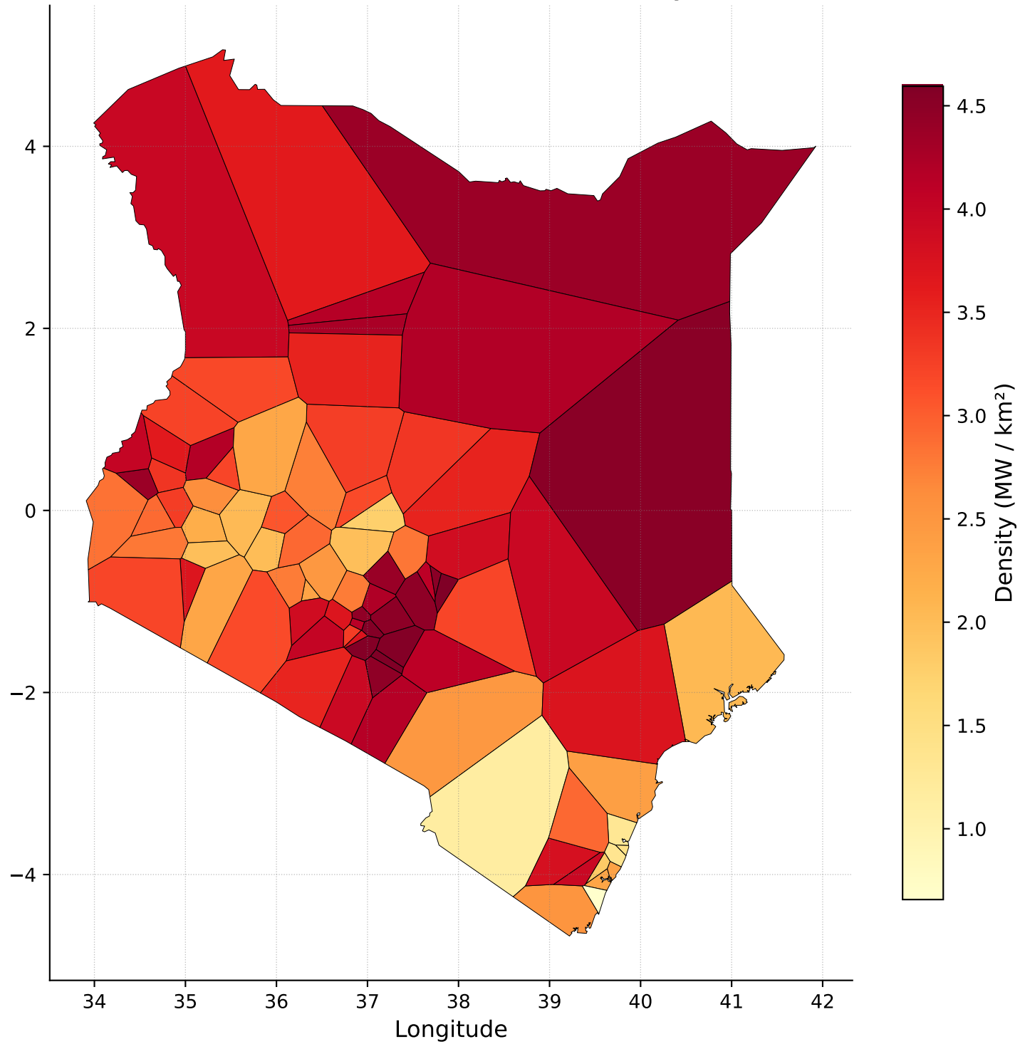
Solar: Voronoi Potential Density
