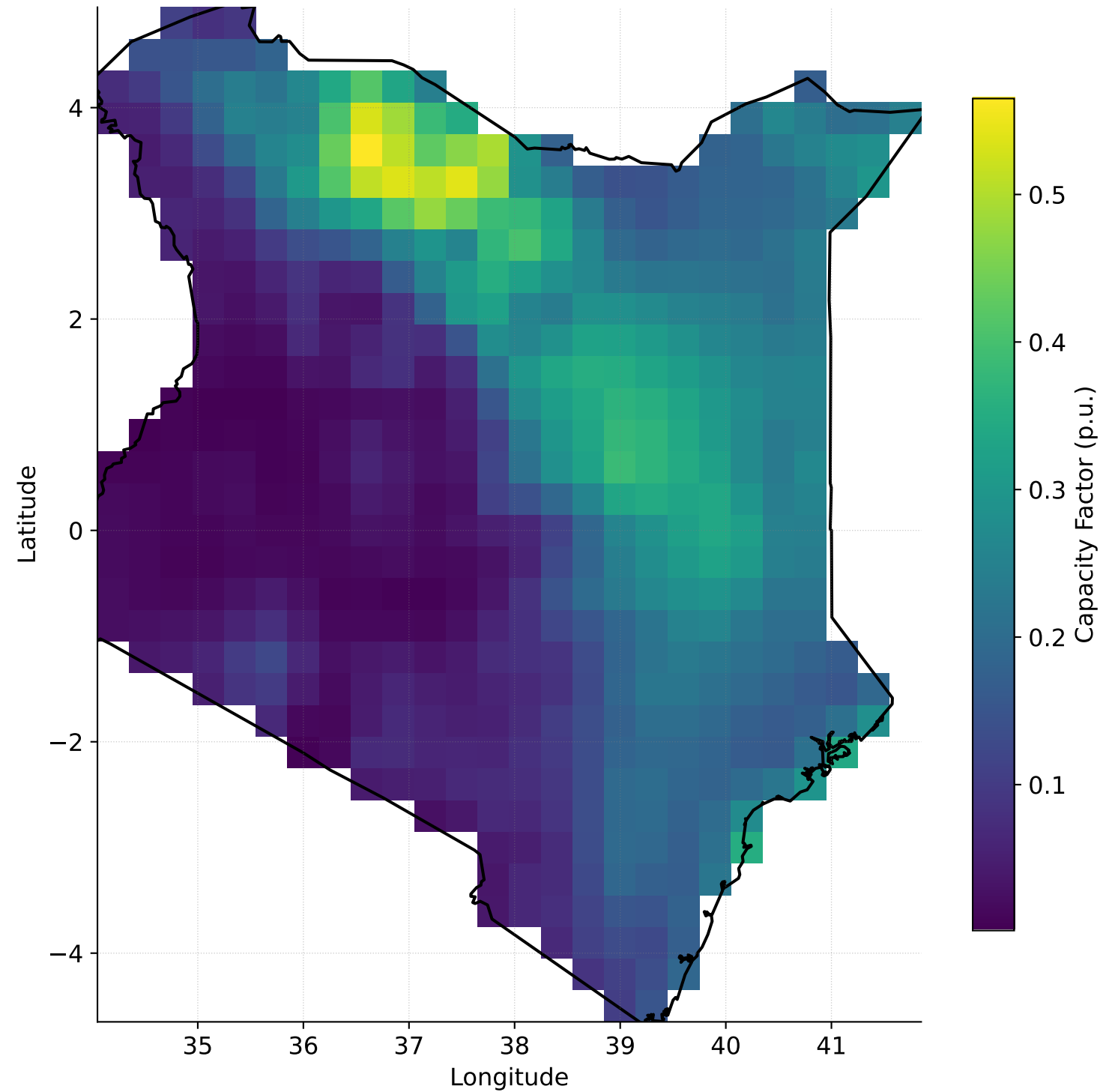
Onshore Wind: Raw High-Res Capacity Factor
