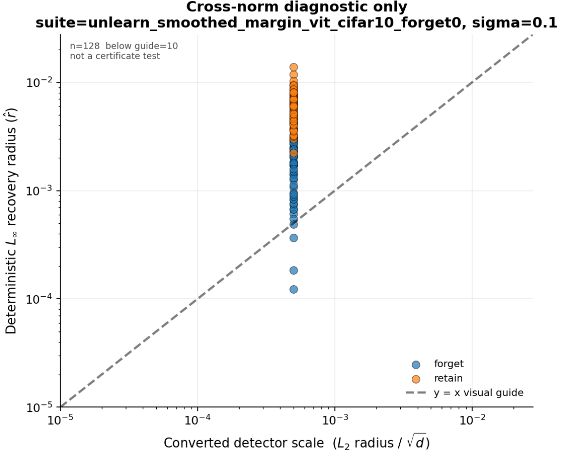
Figure 7: Cross-norm stress diagnostic for the smoothed-margin row (seed 42). This is not a certificate test: it compares a dimension-converted L_2 detector-radius scale to a deterministic base-model L_\infty recovery audit.
