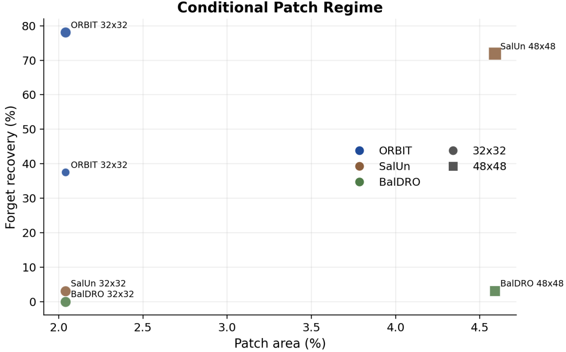
Figure 3: Conditional patch regime. ORBIT admits strong low-area patch recovery, SalUn requires a larger patch and incurs more retain damage, and BalDRO is effectively negative under the same patch family.
