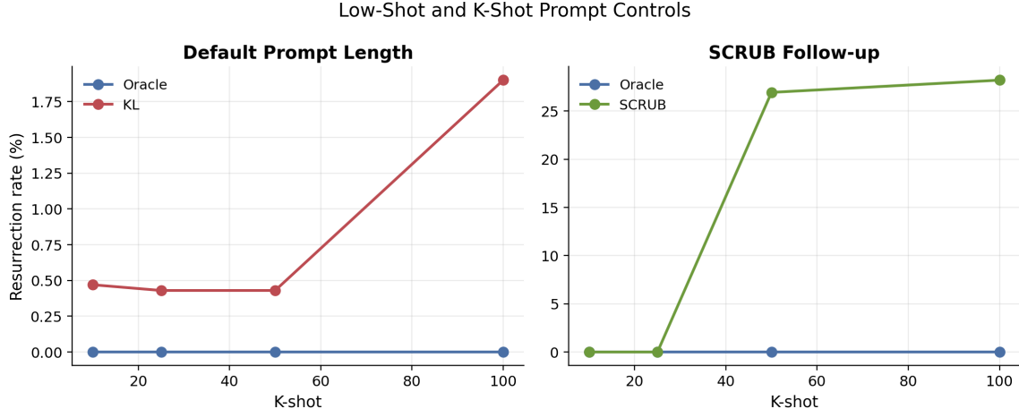
Figure 8: K-shot prompt controls. Oracle stays flat, KL remains weakly vulnerable, and SCRUB only becomes unstable in the larger-shot follow-up.
