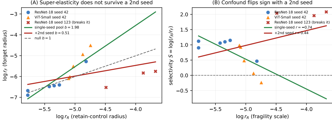
Figure 6: Cross-architecture check on CIFAR-100 (six LoRA unlearning methods per cell), illustrating why the pooling estimator matters. (A) forget-radius log-log fit and (B) the selectivity-fragility confound. Naively pooling raw radii across cells is confounded by their differing fragility baselines: the single-seed pool (circles/triangles) gives \hat{b} = 1.98 , r = -0.74 , but adding the second ResNet-18 seed (red \times ), whose cell is half left-censored at r_F = 0 , flips the raw pooled fit to \hat{b} = 0.51 , r = +0.44 . Within-cell fixed-effects pooling removes this baseline confound and recovers the within-benchmark pattern ( \hat{b} = 1.55 , r = -0.48 ; Section 3.9). The raw cross-cell pool shown here is the wrong estimator; it is retained to make the confound visible.
