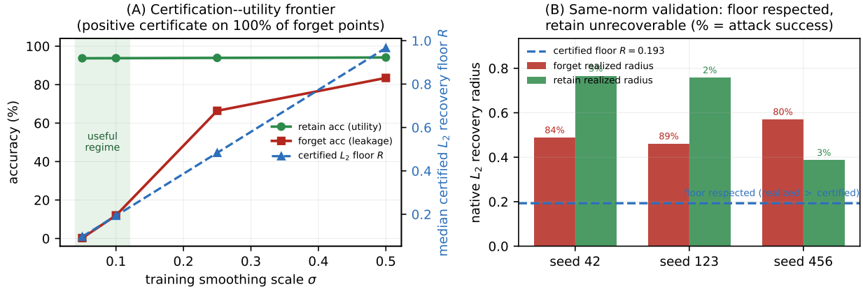
Figure 7: The smoothed-margin objective as a constructive result (Theorem 4). (A) Certification–utility frontier (seed 42): raising the training smoothing scale \sigma grows the median certified L_2 recovery floor R = \sigma \Phi^{-1}(1 - \tau) (right axis, positive certificate on 100% of forget points) while retain accuracy stays flat at \approx 94\% ; strong forgetting lives at small \sigma , so the useful regime is the shaded band and the headline run uses \sigma = 0.10 . (B) Same-norm validation: across seeds 42/123/456 the realized native L_2 forget recovery radius (0.46–0.57) sits above the certified floor R = 0.193 (the floor is respected, not merely consistent), while the retain controls are essentially unrecoverable (attack success 2–3% vs. 80–89% on forget). Deterministic methods carry a certified floor of 0 on this axis. Data: smoothed_margin_sigma_frontier.json , smoothed_margin_l2_recovery_summary.json .
