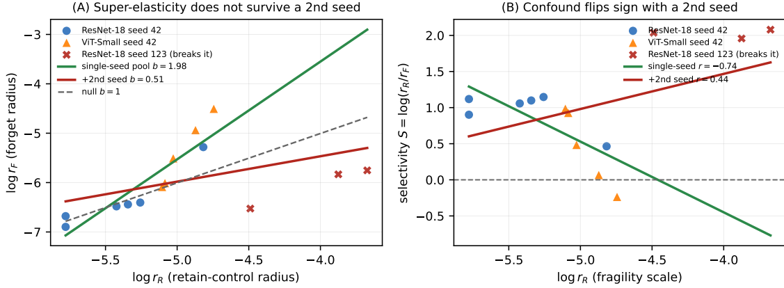
Figure 6: Cross-architecture check on CIFAR-100 (six LoRA unlearning methods per cell), shown as a cautionary negative. On the single-seed-per-cell pool (ResNet-18 and ViT-Small, both seed 42; circles and triangles) (A) the forget-radius log-log fit has slope \hat{b} = 1.98 (green) and (B) the selectivity–fragility confound is r = -0.74 (green), both signed like the within-benchmark mechanism. This agreement is not robust : the second ResNet-18 seed (red \times ) lands in a high- r_R /high-selectivity regime that the confound predicts should be empty, flipping the pooled fit to \hat{b} = 0.51 and r = +0.44 (red). Cross-architecture generalization of these effects is therefore not established; the robust evidence is within-benchmark (three seeds) and the controlled causal experiment.
