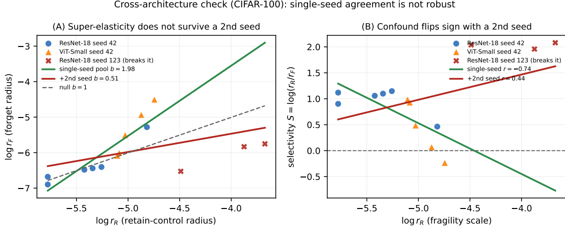
Figure 6: Cross-architecture check on CIFAR-100 (six LoRA unlearning methods per cell), illustrating why the pooling estimator matters. (A) forget-radius log-log fit and (B) the selectivity–fragility confound. Naively pooling raw radii across cells is confounded by their differing fragility baselines: the single-seed pool (circles/triangles) gives \hat{b} = 1.98 , r = -0.74 , but adding the second ResNet-18 seed (red \times ), whose cell is half left-censored at r_F=0 , flips the raw pooled fit to \hat{b} = 0.51 , r = +0.44 . Within-cell fixed-effects pooling removes this baseline confound and recovers the within-benchmark pattern ( \hat{b} = 1.55 , r = -0.48 ; Section 3.9). The raw cross-cell pool shown here is the wrong estimator; it is retained to make the confound visible.
