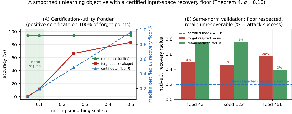
Figure 7: The smoothed-margin objective as a constructive result (Theorem 4). (A) Certification-utility frontier (seed 42): raising the training smoothing scale \sigma grows the median certified L_2 recovery floor R = \sigma \Phi^{-1}(1 - \tau) (right axis, positive certificate on 100% of forget points) while retain accuracy stays flat at \approx 94\% ; strong forgetting lives at small \sigma , so the useful regime is the shaded band and the headline run uses \sigma = 0.10 . (B) Same-norm validation: across seeds 42/123/456 the realized native L_2 forget recovery radius (0.46–0.57) sits above the certified floor R = 0.193 (the floor is respected, not merely consistent), while the retain controls are essentially unrecoverable (attack success 2–3% vs. 80–89% on forget). Deterministic methods carry a certified floor of 0 on this axis. Data: smoothed_margin_sigma_frontier.json , smoothed_margin_l2_recovery_summary.json .
