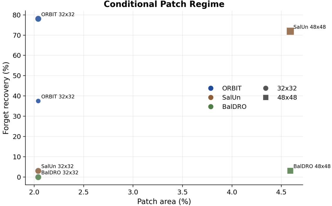
Figure 4: Conditional patch regime. ORBIT admits strong low-area patch recovery, SalUn requires a larger patch and incurs more retain damage, and BalDRO is effectively negative under the same patch family.
