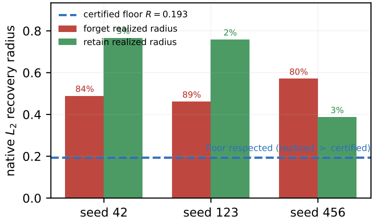
(B) Same-norm validation: floor respected, retain unrecoverable (% = attack success)
