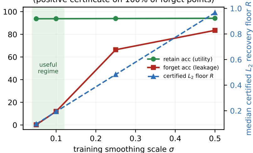
(A) Certification--utility frontier (positive certificate on 100% of forget points)
