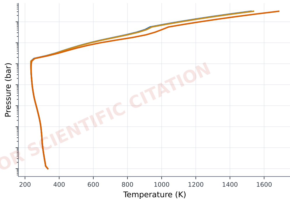
Virga cloudy, f sed =3 · 100× solar
