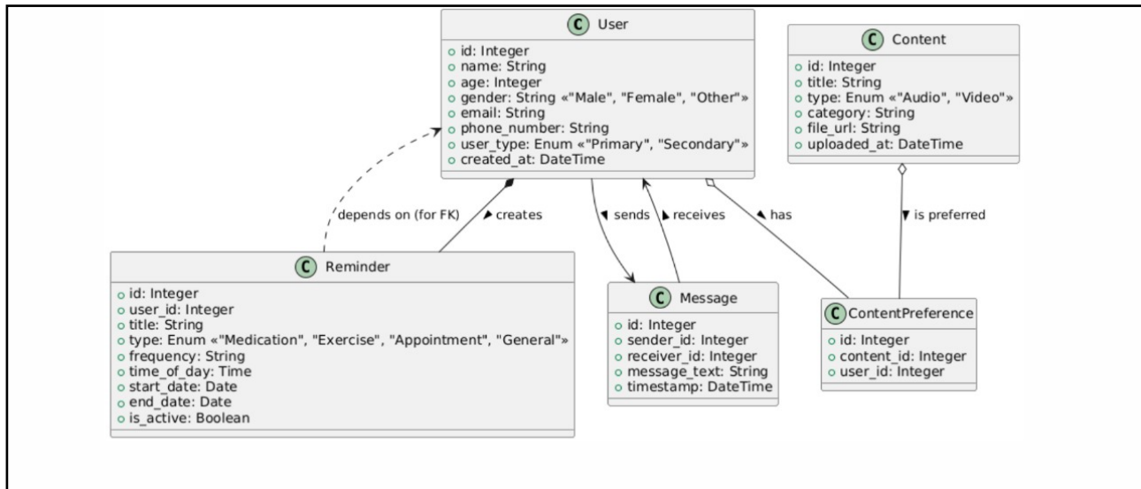
Image 3 shows the class diagram for the app.
