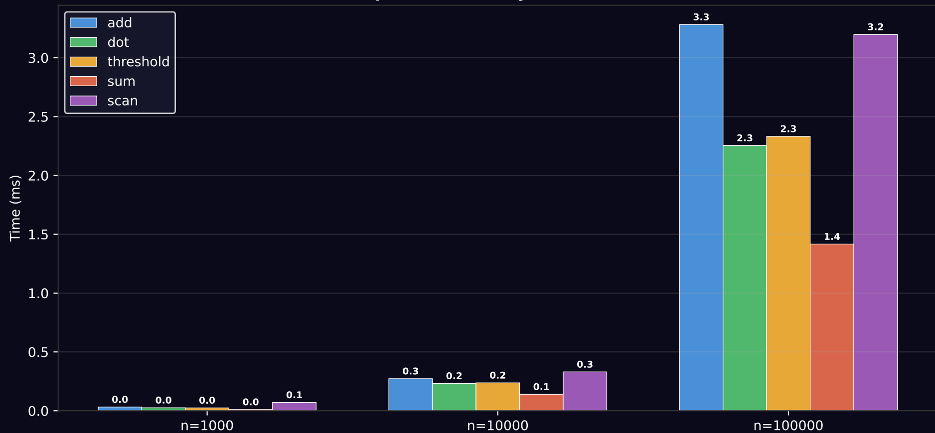
Operation Time by Vector Size
