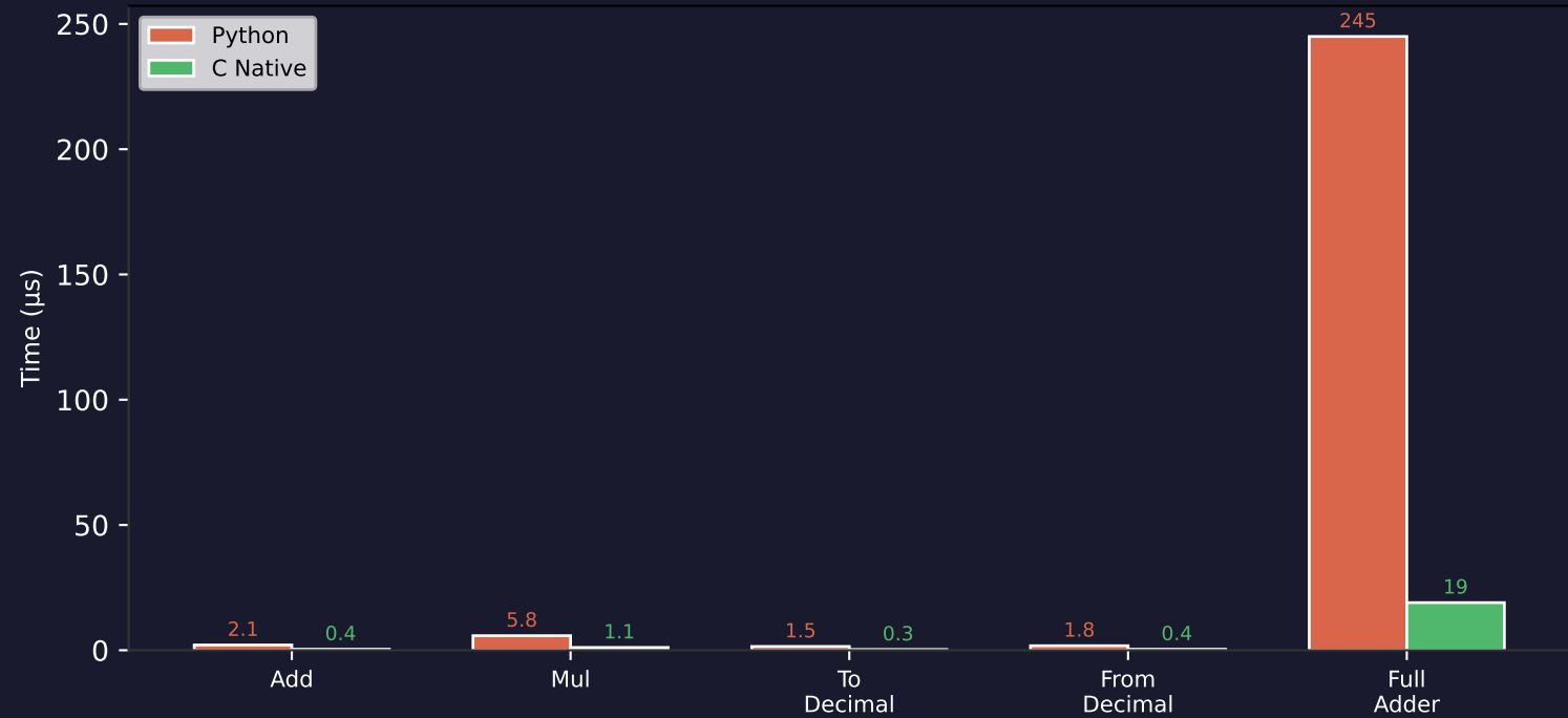
Python vs C Native: 1M Operations (lower is better)
