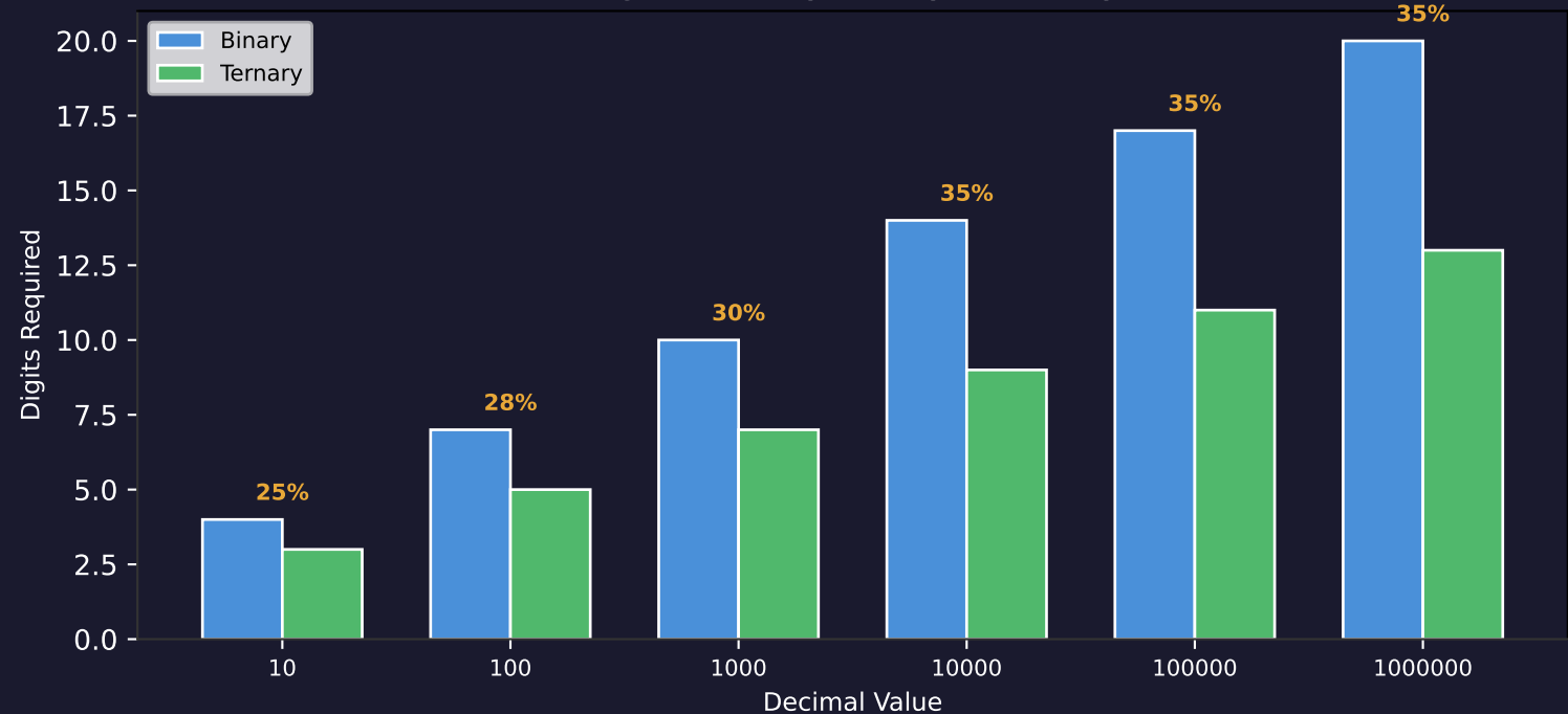
Digit Efficiency: Binary vs Ternary
