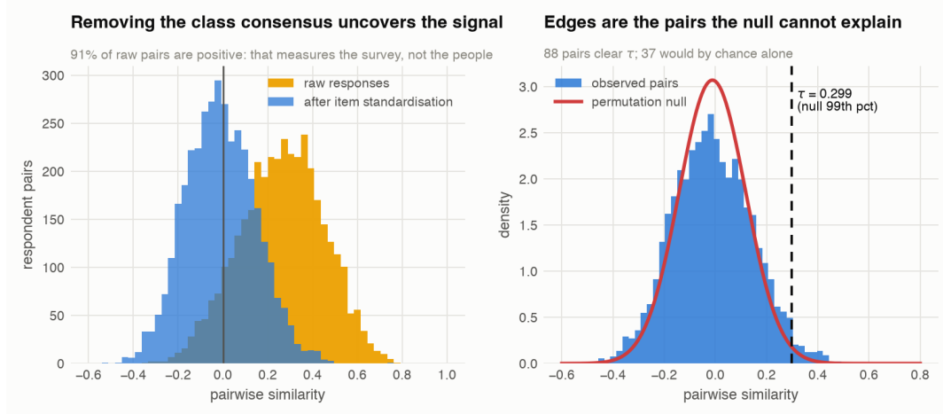
Figure 2: Left: subtracting the class consensus moves the similarity distribution from “almost everything is positive” to centred on zero. Right: the edge threshold is the 99th percentile of a permutation null, not a hand-picked number.
