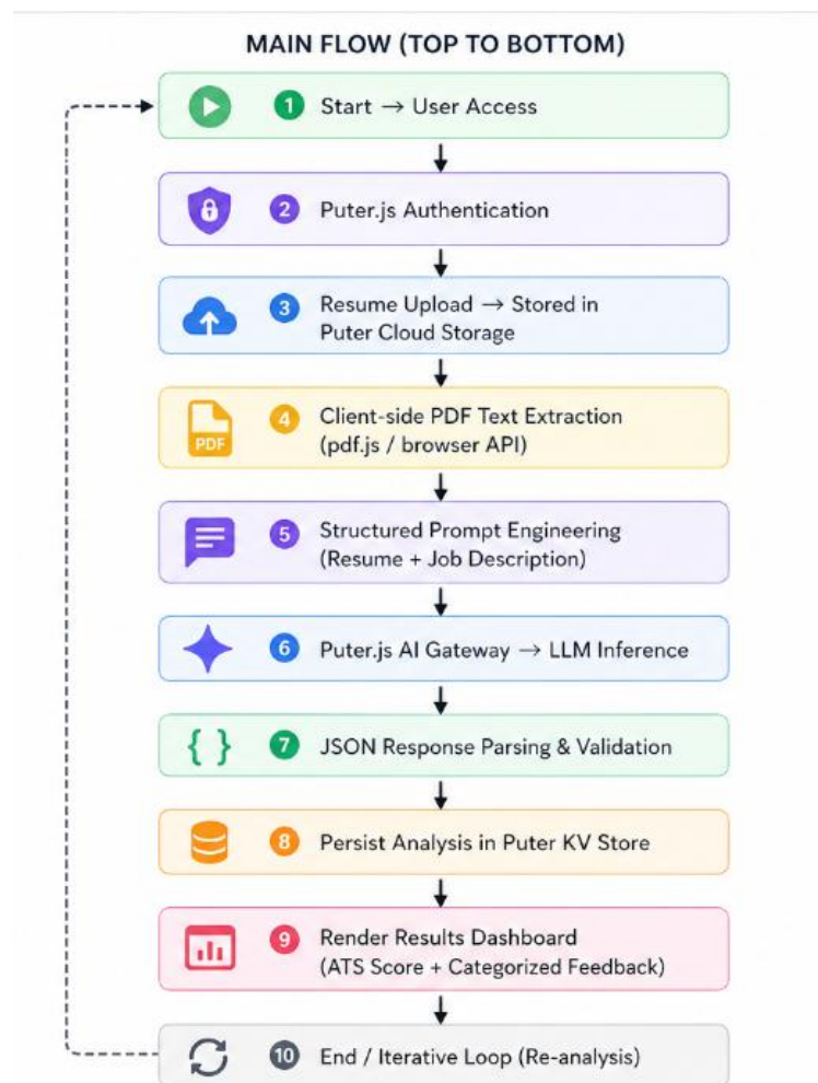
Figure 3-3: Activity Diagram
