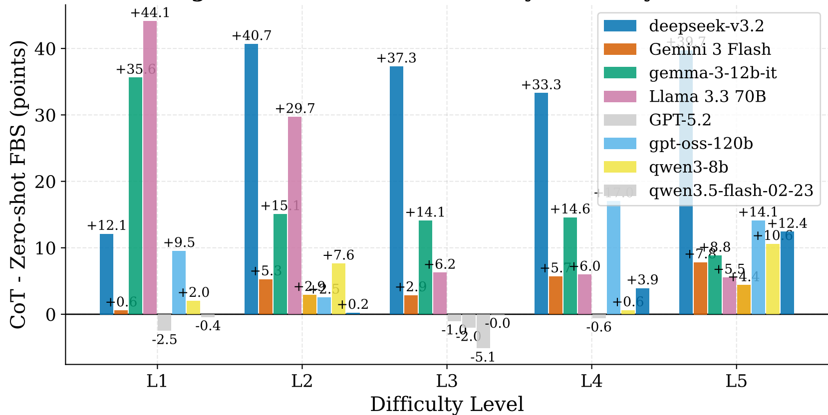
Figure 6: CoT Effect on FBS by Difficulty Level
