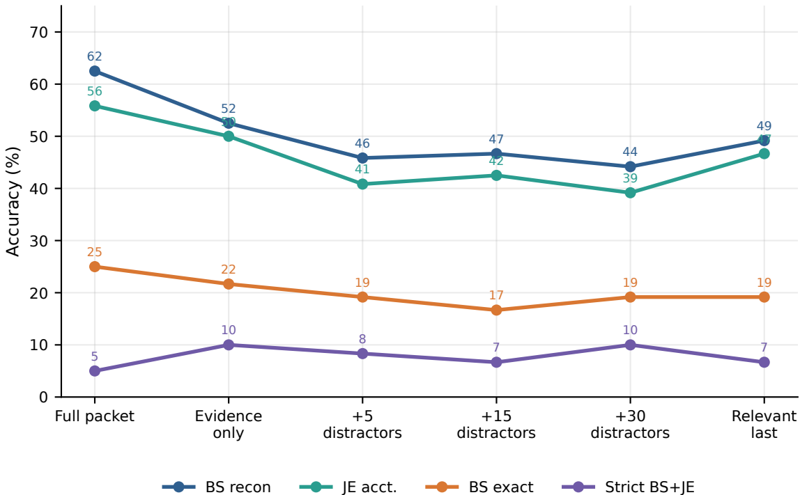
Context Stress: Evidence Ordering and Added Distractors
