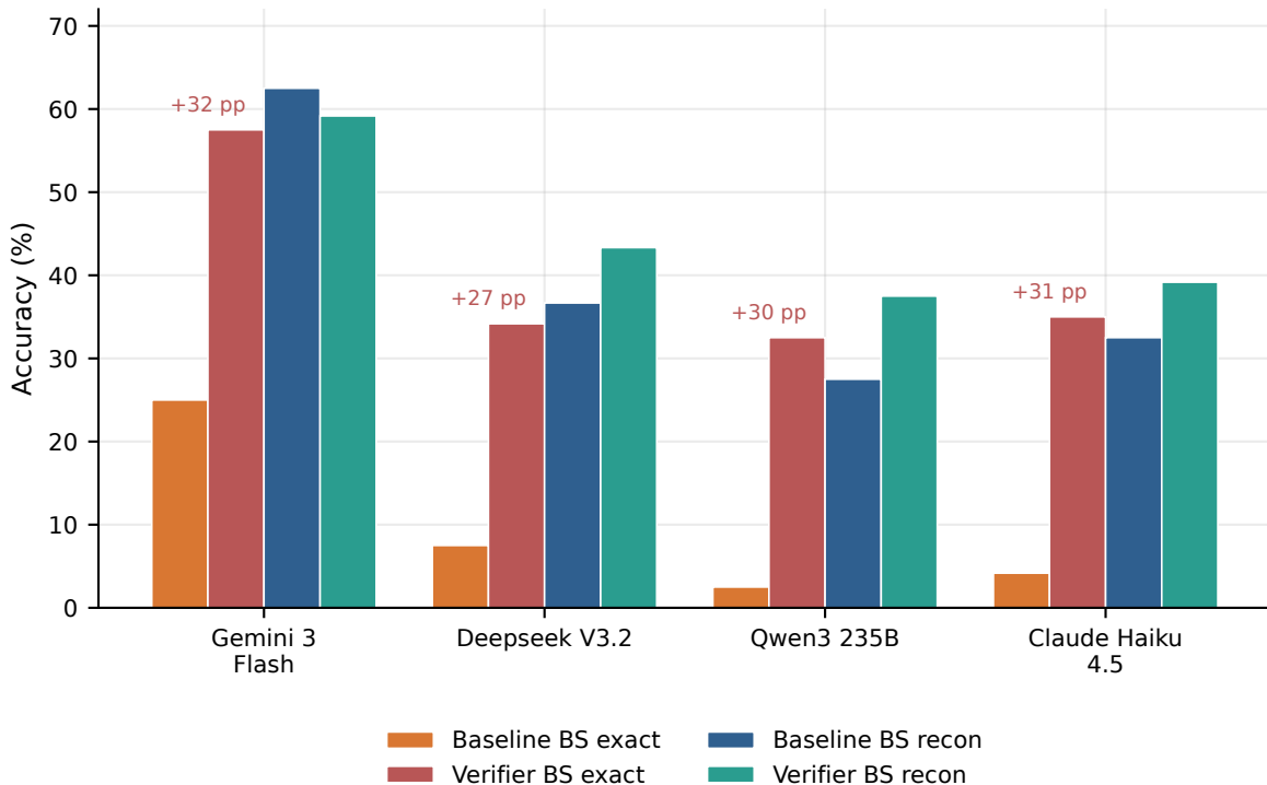
Forced Ledger Verifier Transfers Across Models
