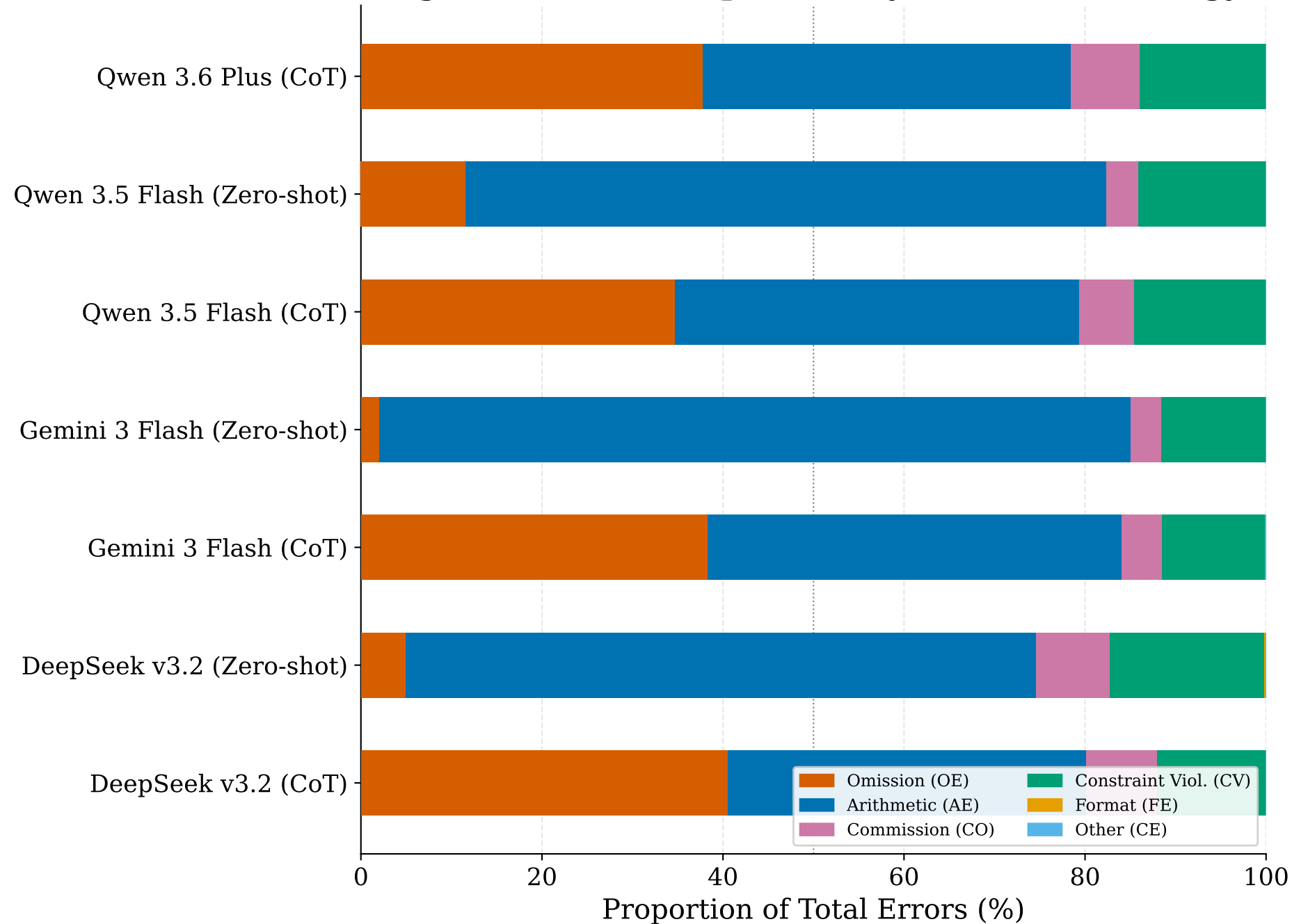
Figure 2: Error Composition by Model and Strategy
