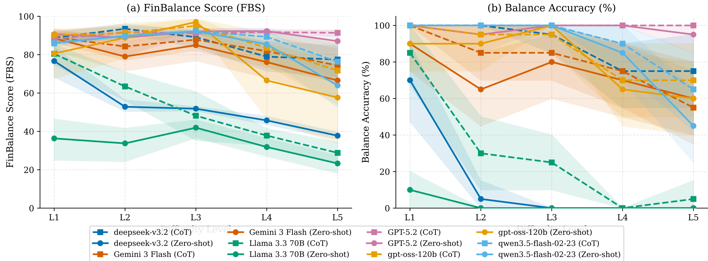
Figure 1: Performance vs. Difficulty Level (Capability Curve)
