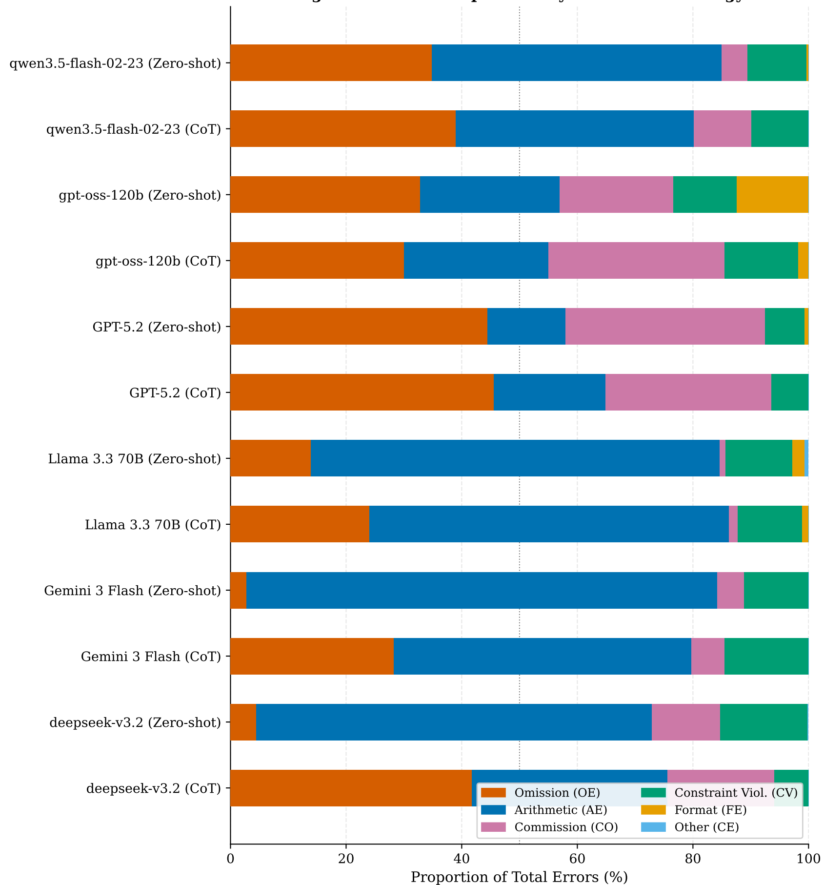
Figure 2: Error Composition by Model and Strategy
