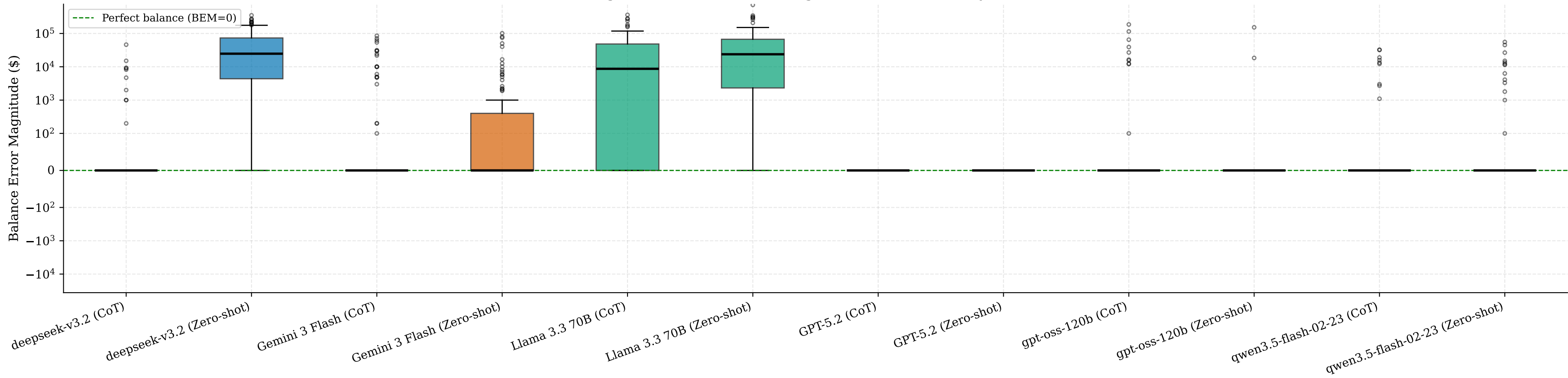
Figure 5: Balance Error Magnitude Distribution by Model
