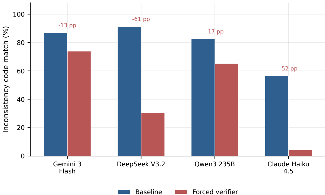
Ledger Verifier Trade-off on Inconsistency Detection
