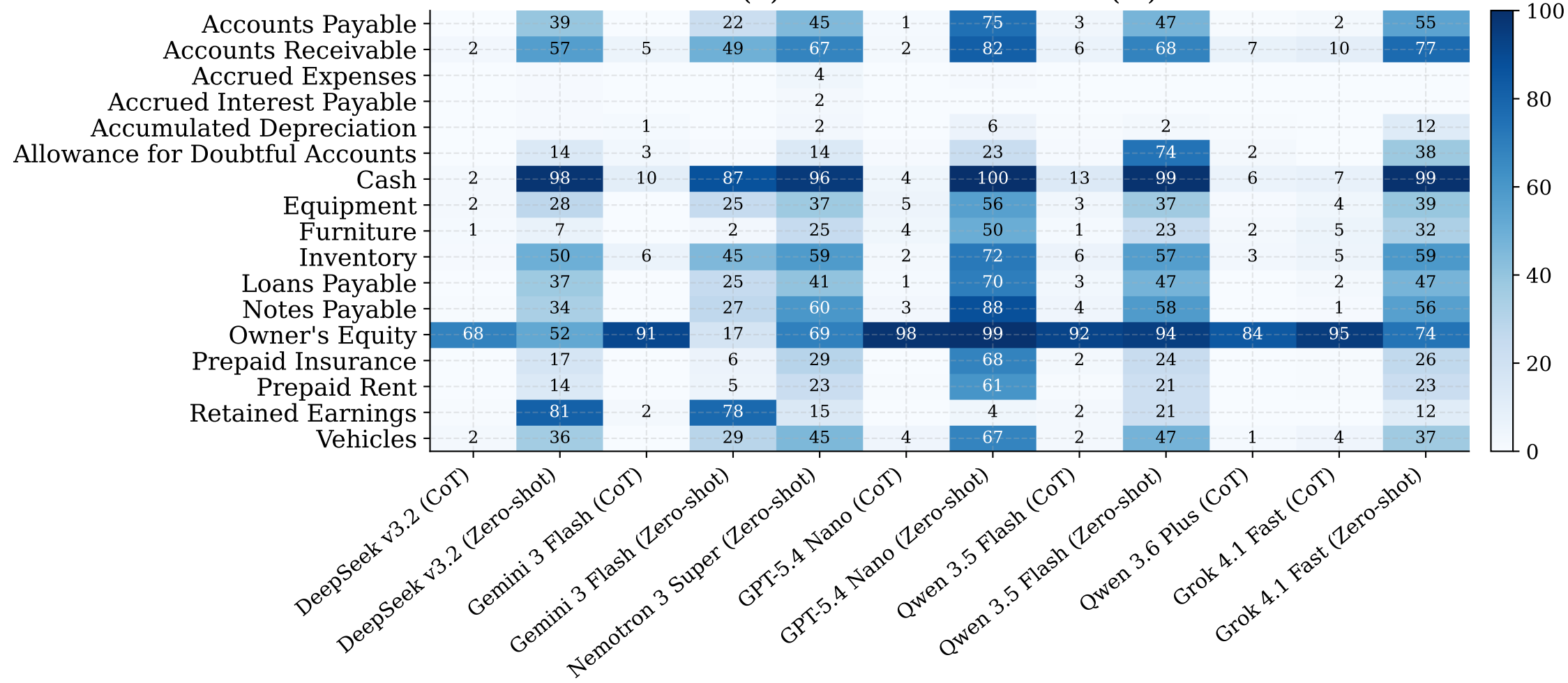
(b) Arithmetic Error Rate (%)
