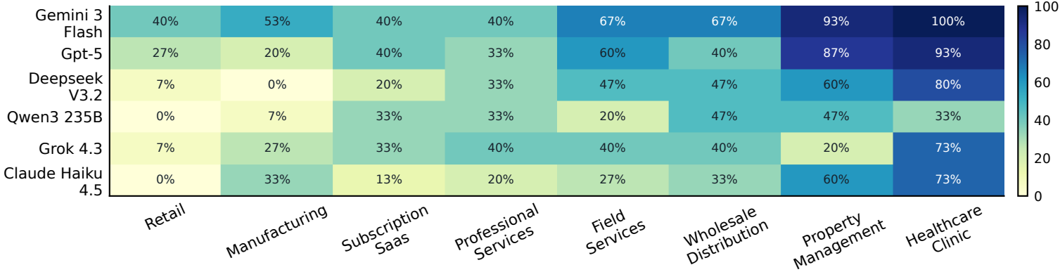
BS Recon Accuracy by Ledger Family
