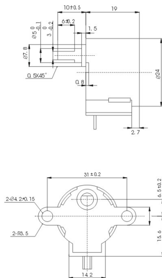
24BYJ48
