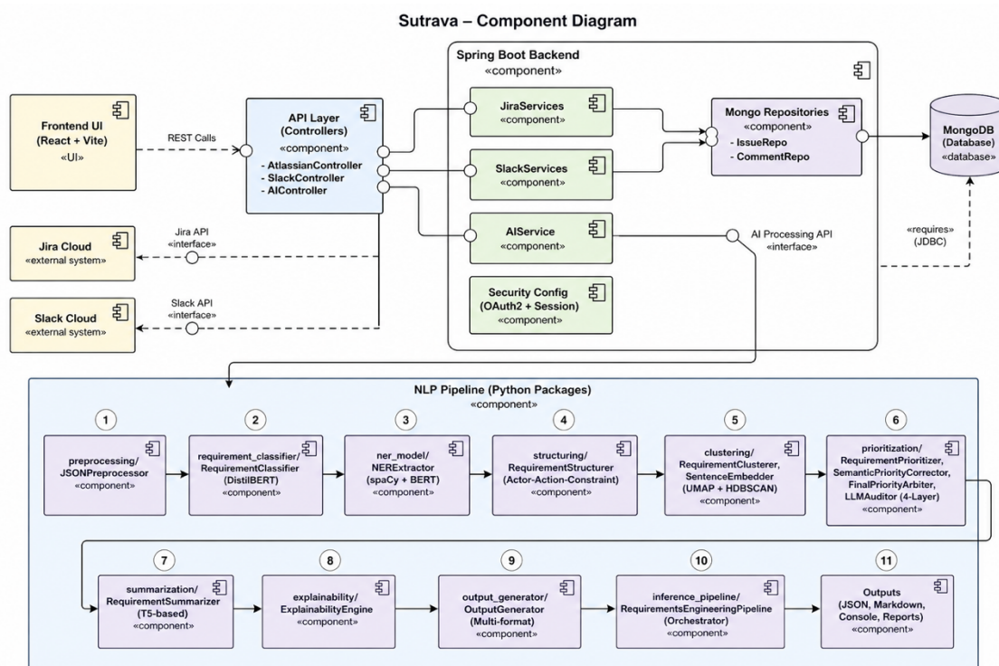
Fig. 3.4: Component Diagram
