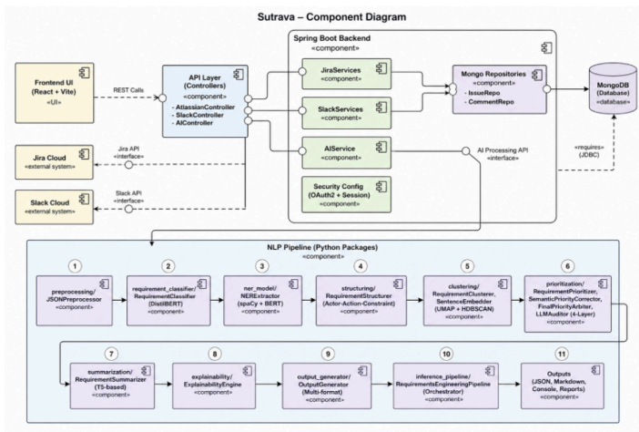
Fig. 3.4: Component Diagram
