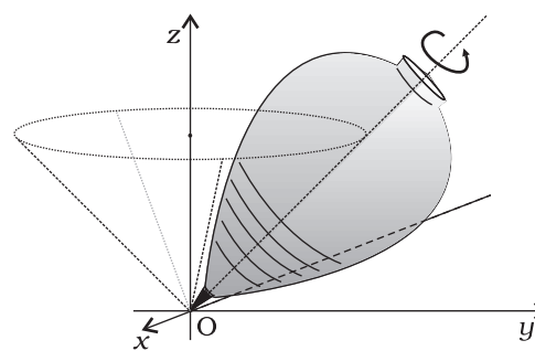
Fig. 7.5 (a) A spinning top (The point of contact of the top with the ground, its tip O, is fixed.)
