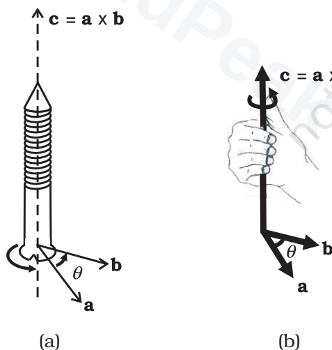
Fig. 7.15 (a) Rule of the right handed screw for defining the direction of the vector product of two vectors.
