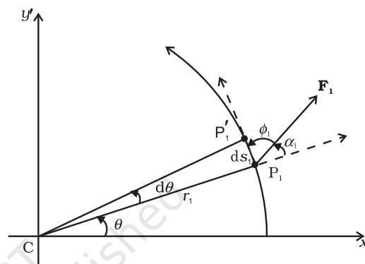
Fig. 7.34 Work done by a force \mathbf{F}_1 acting on a particle of a body rotating about a fixed axis; the particle describes a circular path with centre C on the axis; arc P_1P'_1(ds_1) gives the displacement of the particle.
