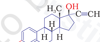
Ethynylestradiol (novestrol)
