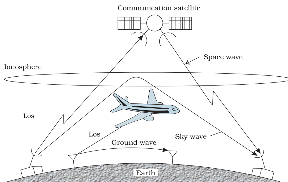
FIGURE 15.6 Various propagation modes for em waves.
