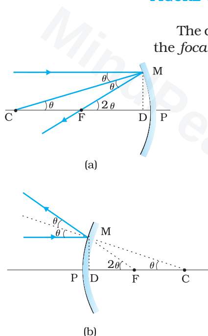
FIGURE 9.4 Geometry of reflection of an incident ray on (a) concave spherical mirror, and (b) convex spherical mirror.
