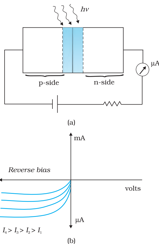
FIGURE 14.23 (a) An illuminated photodiode under reverse bias, (b) I - V characteristics of a photodiode for different illumination intensity I_4 > I_3 > I_2 > I_1 .
