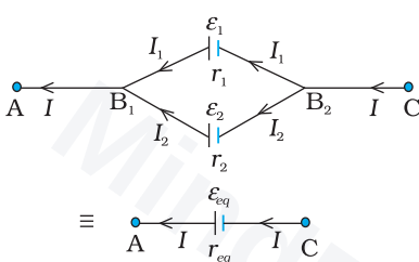
FIGURE 3.21 Two cells in parallel. For connections across A and C, the combination can be replaced by one cell of emf \varepsilon_{eq} and internal resistances r_{eq} whose values are given in Eqs. (3.73) and (3.74).
