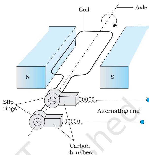
FIGURE 6.16 AC Generator
