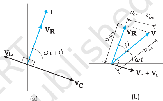
FIGURE 7.13 (a) Relation between the phasors \mathbf{V}_L , \mathbf{V}_R , \mathbf{V}_C , and \mathbf{I} , (b) Relation between the phasors \mathbf{V}_L , \mathbf{V}_R , and (\mathbf{V}_L + \mathbf{V}_C) for the circuit in Fig. 7.11.
