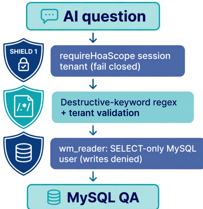
Fig. 2 - Even a malicious prompt can only call a closed function with validated params.
