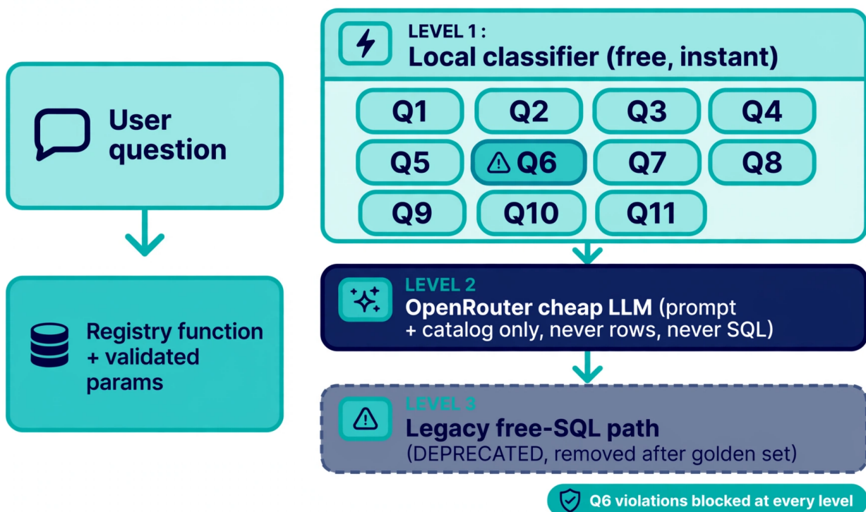
Fig. 5 - Cascade: local -> cheap LLM -> legacy (deprecated).
