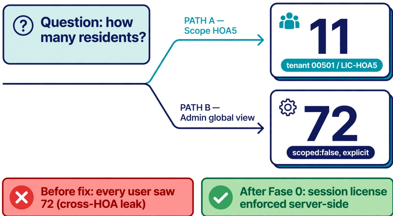
Fig. 1 - Tenant isolation proof: HOA5 sees 11, global sees 72.
