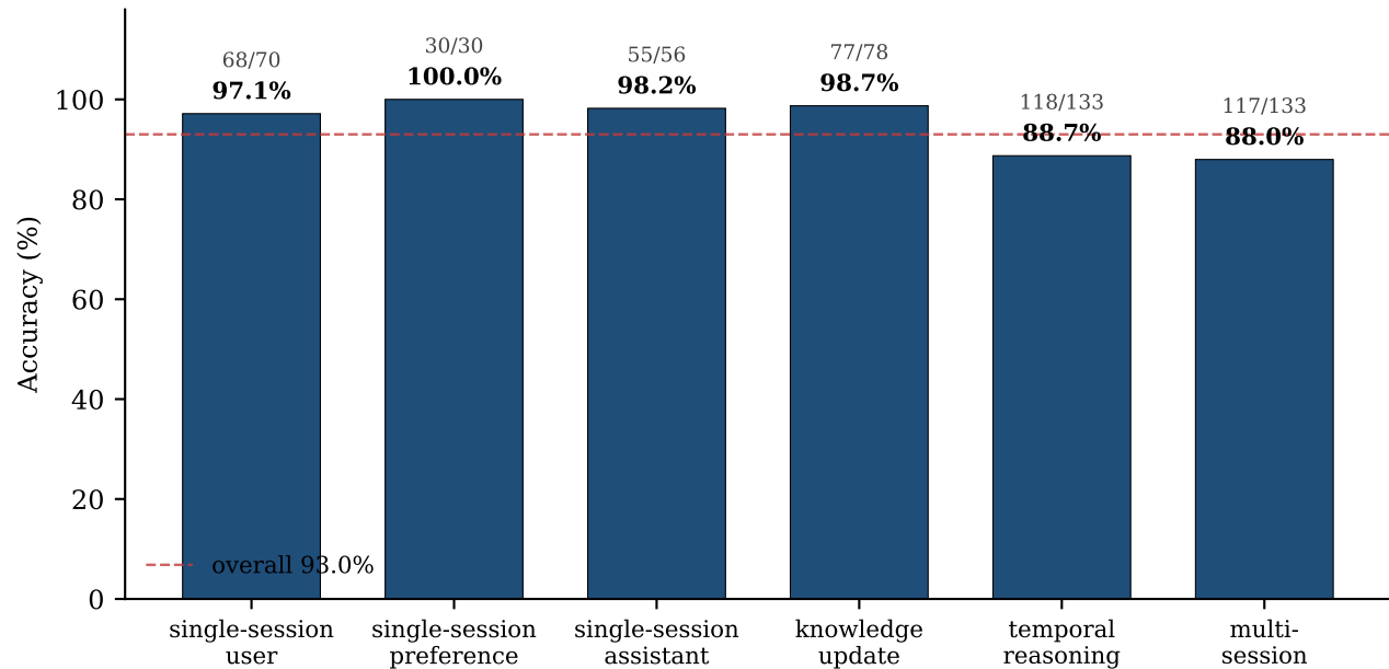
LongMemEval-500 per-category accuracy (Azure gpt-5.4, 2026-04-24)
