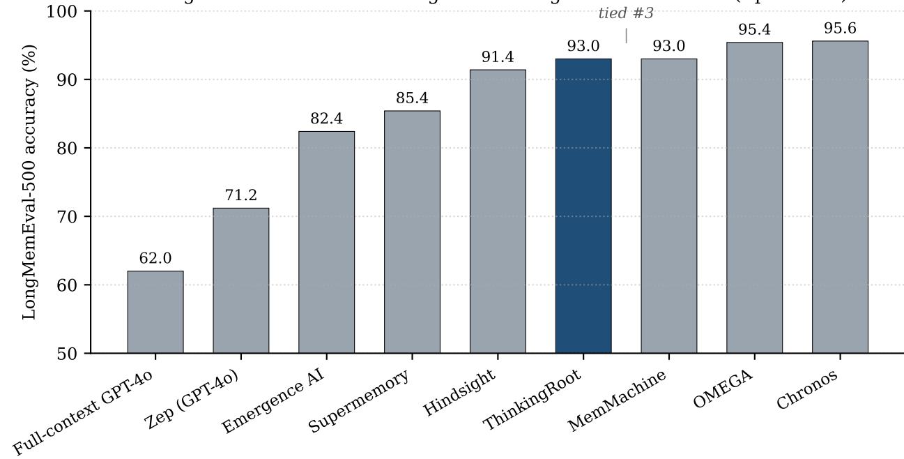
LongMemEval-500 — ThinkingRoot in the global leaderboard (April 2026)
