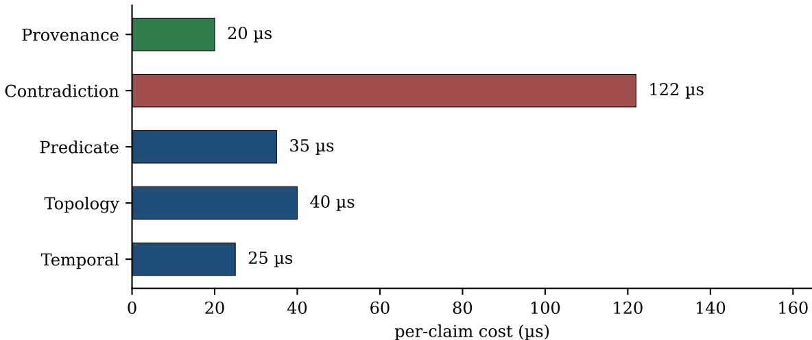
Rooting probe cost (divan, N = 100 \rightarrow 242 \mu\text{s} total)
