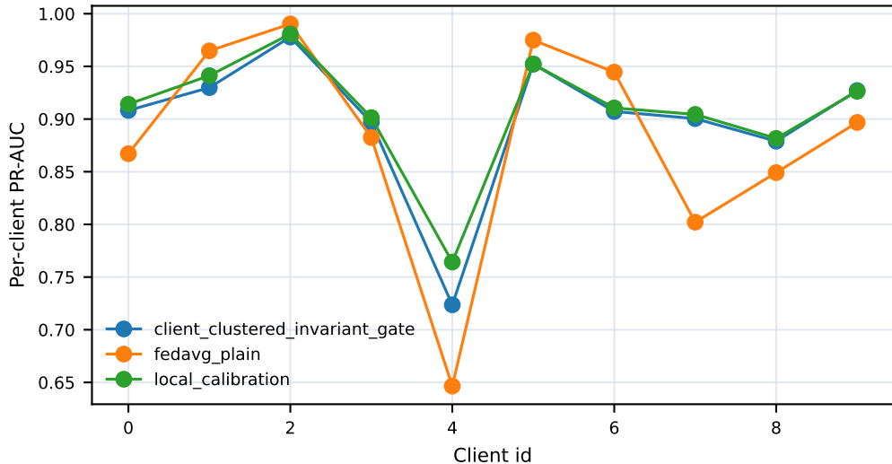
VCSL public-label client variability
